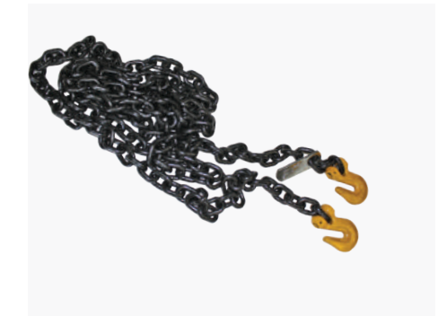
GRADE 80 CHAIN ACC-CHAN | 16' ACC-CHAN-20 | 20' This rugged chain is 3/8"/1 cm with grab hooks and a WLL of 7,100 lbs/3,227 kg, this chain is approved for overhead lifting. Available in 16'/5 m or 20'/6 m lengths.
